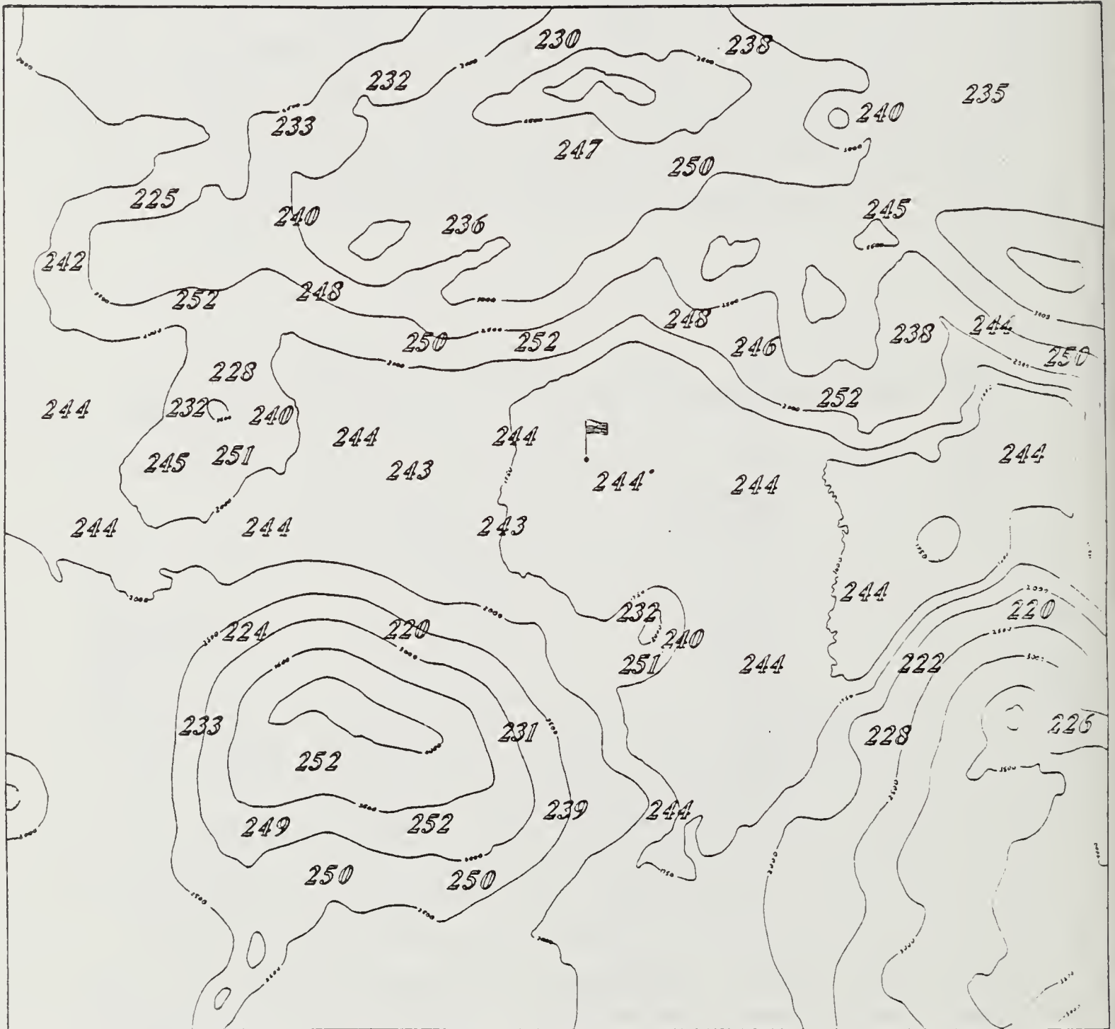
Mean surface temperature ( ^{\circ} K) in the region of Taurus Littrow. The contours represent topography.
